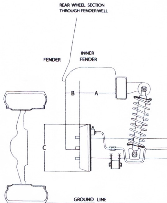
Rear Drum Brake
