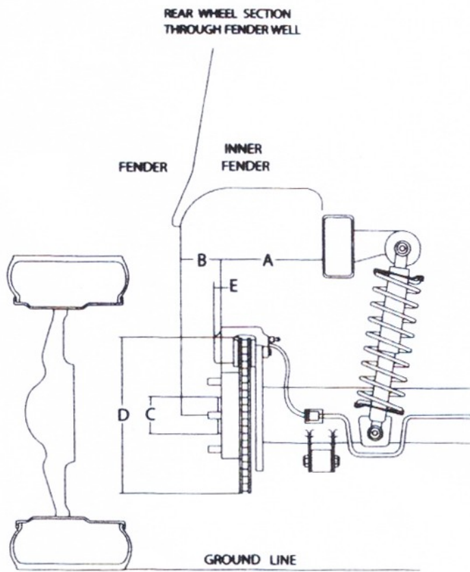
Rear Disk Brake
